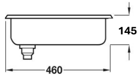
Single bowl with drainer Single bowl inset sink SS-120-950-508-REV 0.6 Gauge
